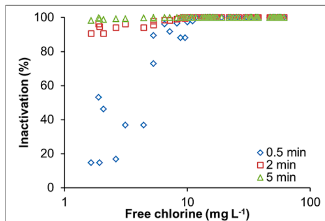
Figure 3. Inactivation of bacteria collected from aviary hen house treated with MLAEW at different free chlorine concentrations, and treatment time 0.5, 2 or 5 min
