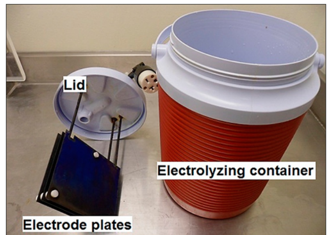
Figure 1. Electrolyzing container and components
