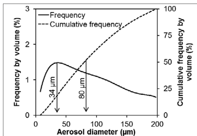
Figure 2. Aerosol size distribution (nebulized using spray gun with 0.5 mm nozzle at 1.4 bar)
