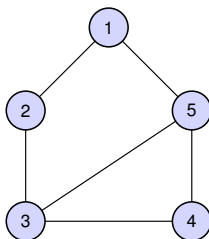
Fig. 1. Communication graph.
