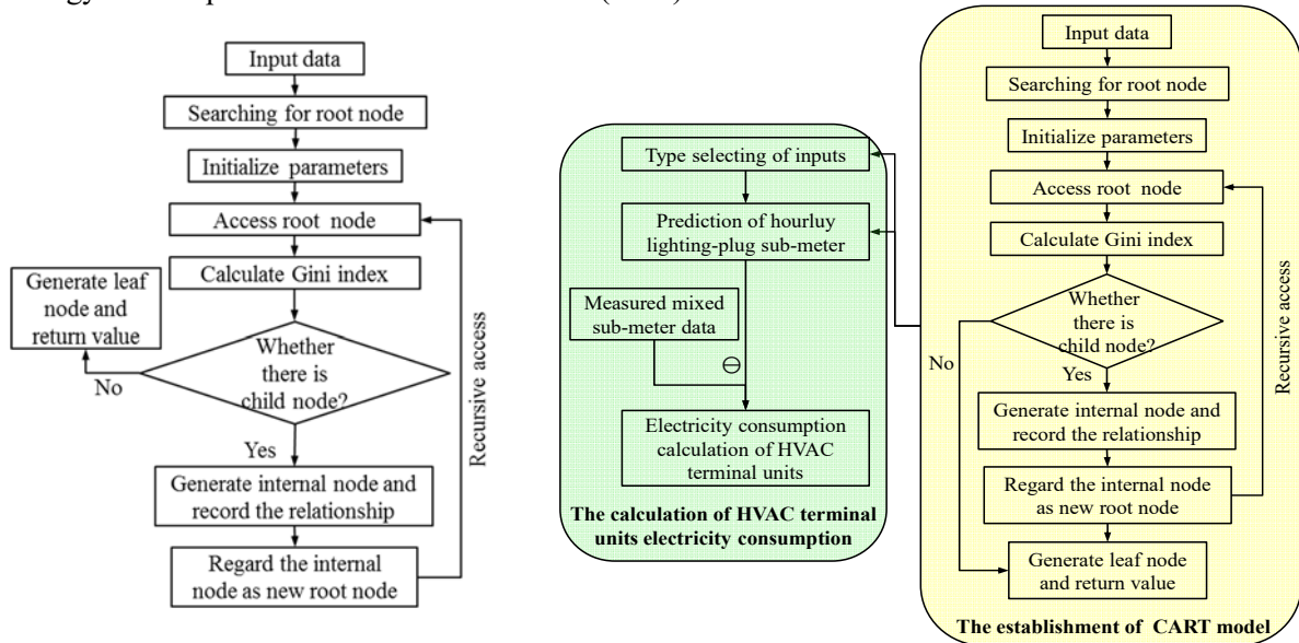
Figure 1. The establishment procedure of a tree model with CART algorithm Figure 2. The model for calculating hourly electricity consumption of HVAC terminal units
