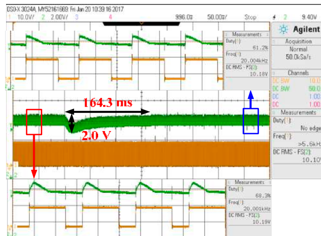
(a) Conventional PI control
