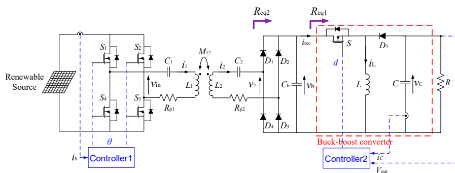
Figure 7. Schematic diagram of a typical two-stage SS-compensated wireless power transfer (WPT) system.
