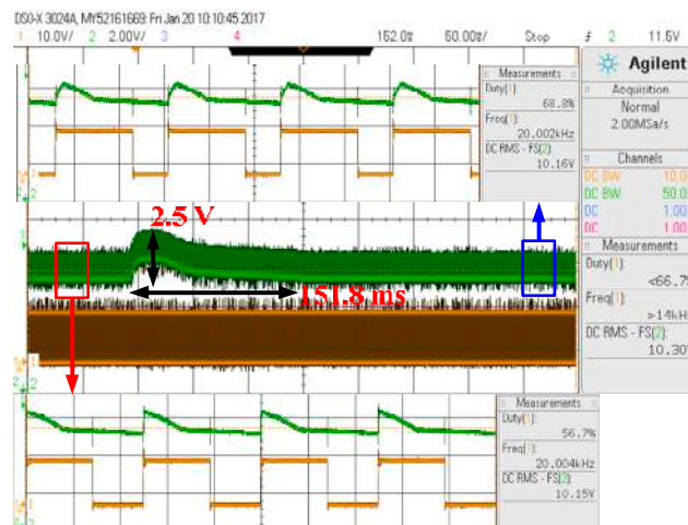
(a) Conventional PI control
