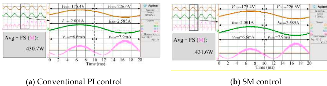
Figure 2. The experimental waveforms of the output voltage, the output current, and the output power of wind turbine system for wind speed altering from 6.6 to 7.9 m/s.
