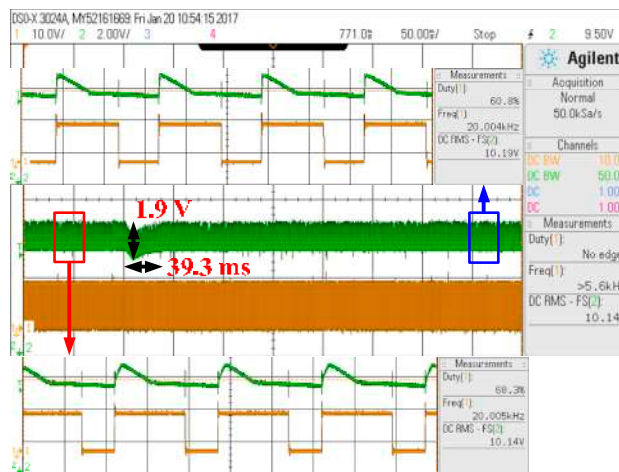
(b) SM control
