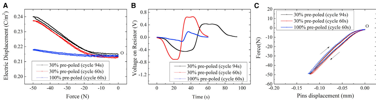
Figure 4. Quasi-static cycles with 4.620-M \Omega resistive load
