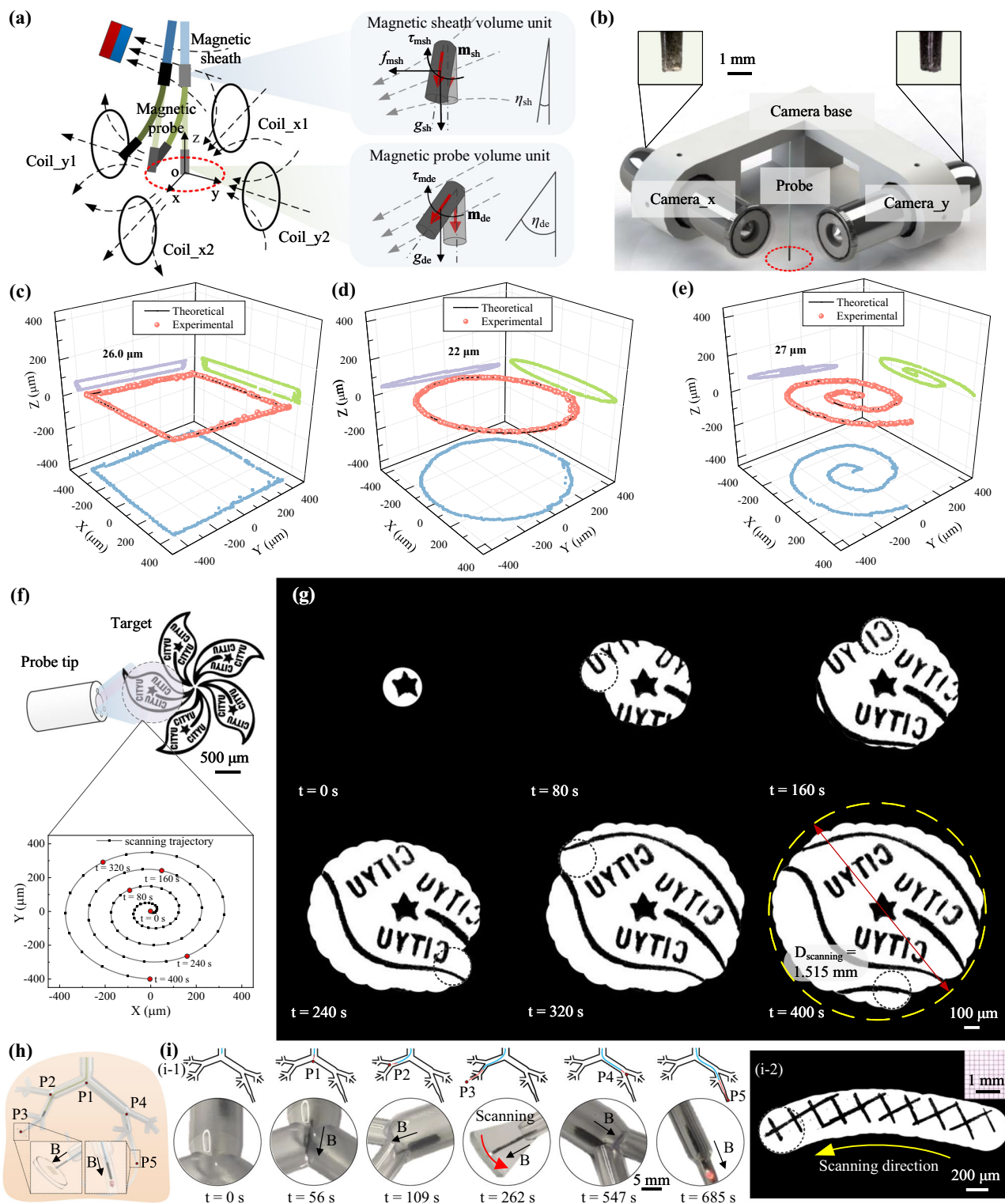
Fig. 4 | High precise maneuvering of the continuum robot. a Schematic depicting the multi-sectional actuation by the magnetic field. The magnetic sheath is actuated by a gradient magnetic field to achieve large-range steering, while the magnetic probe is actuated by a uniform magnetic field to achieve high-precision motion. b Experimental setup for evaluating the probe's motion trajectory. Path tracking results of the probe tip under square ( c ), circle ( d ), and spiral ( e ) trajectories, presenting a motion error of less than 30 \mu\text{m} for complex 3D trajectories. The light blue, green, and purple dots here correspond to the projection in the x-o-y
