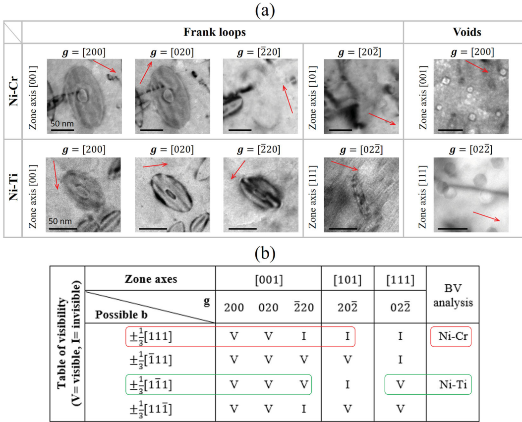
Figure 2. (a) Bright-field TEM images of irradiated Ni-Cr and Ni-Ti (close to surface) under different two-beam conditions with diffraction vector \mathbf{g} indicated by the red arrows with scale bar in each image denotes 50 nm; (b) table of visibility for both outer and inner loops.
