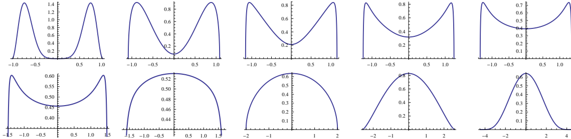
Figure 1: Plots of the q -ultraspherical measure w(\lambda_q x, \beta | q) in (4.4) with \lambda_q = \sqrt{1 - q} and \beta = 0.5 . In the first row, q is negative and increases from -0.9 to -0.1 with a step size 0.2 . While in the second row, q is positive and increases from 0.1 to 0.9 with a step size 0.2 .
