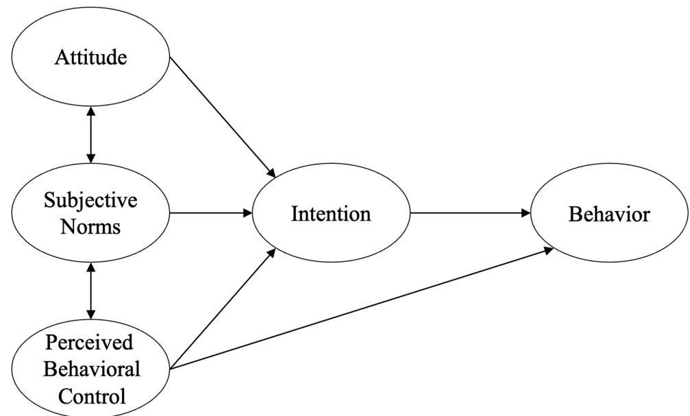
Figure 1. TPB model [92].
