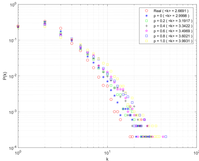
FIGURE 7. Adaptive Degree distribution of the proposed model with varying probabilities of the third Henneberg's edge. The legend in the graph shows the average degree of each network.
