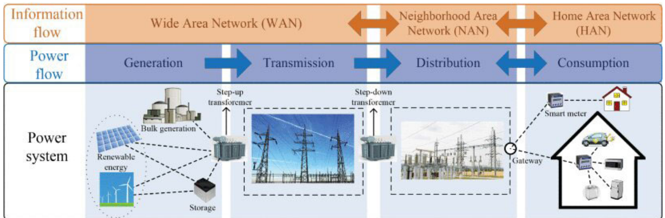
FIGURE 2. Smart grid architecture presenting power systems, power flow, and information flow [5].
