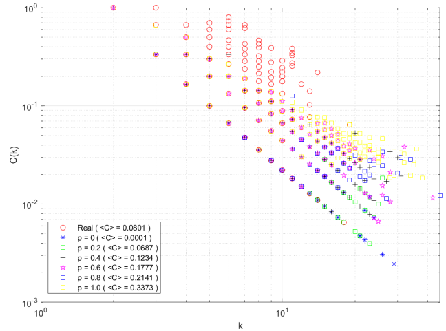
FIGURE 8. Adaptive Clustering Coefficient of the proposed model with varying probabilities of the third Henneberg's edge. The legend in the graph shows the average clustering coefficient of each network.
