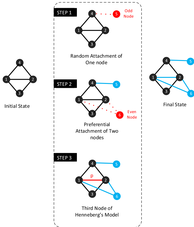
FIGURE 5. Proposed model for power grid networks, powerX. Addition of Odd and Even nodes are shown in STEP 1 and STEP 2. Step 3 shows the interconnection of the third Henneberg's node with probability p .
