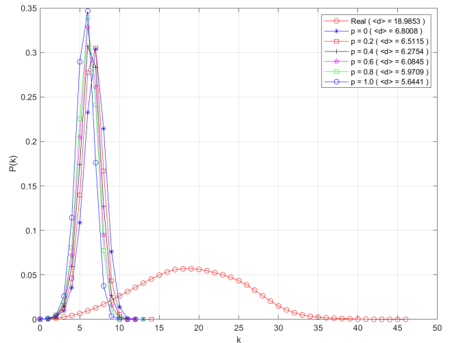
FIGURE 9. Adaptive Distance distribution of the proposed model with varying probabilities of the third Henneberg's edge. The legend in the graph shows the average distance of each network.
