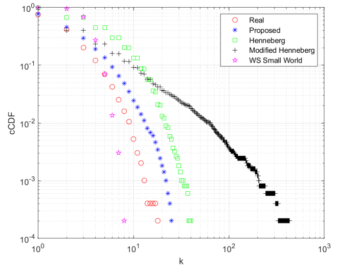
FIGURE 13. Complementary Cumulative Distribution function (cCDF) of the real dataset (US Western States Power Grid), the proposed model, Henneberg's Model, Modified Henneberg's Model, and WS Small World Model.
