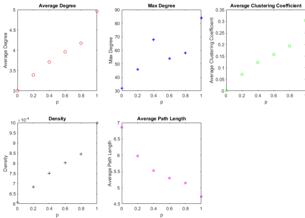
FIGURE 10. Adaptive parameters of the proposed model by changing the probability of the Henneberg's edge.
