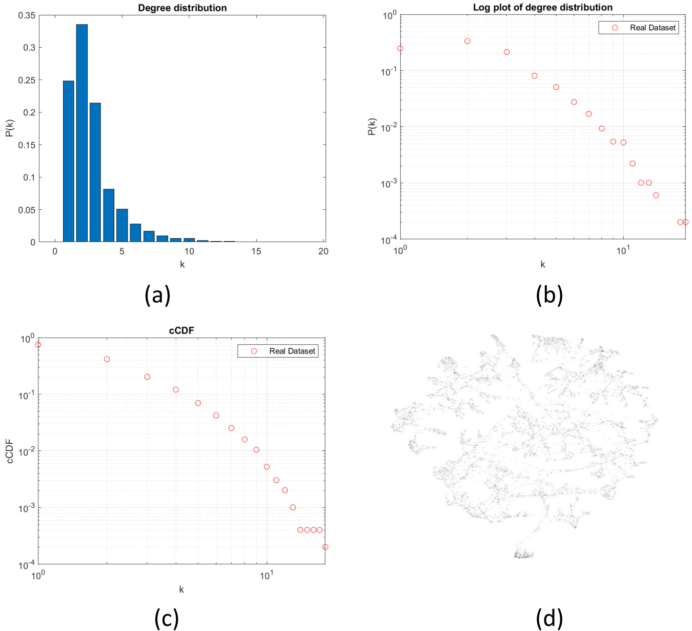
FIGURE 4. Characteristics of the Western States Power Grid network. (a) Degree distribution of the overall network. (b) Log plot of the degree distribution. (c) complementary Cumulative Distribution Function (cCDF). (d) Topological structure of the network constructed using Gephi by the Force Atlas Layout.
