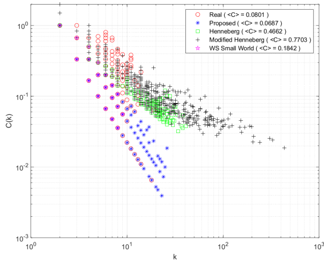
FIGURE 14. Clustering Coefficient of the real dataset (US Western States Power Grid), the proposed model, Henneberg’s Model, Modified Henneberg’s Model, and WS Small World Model. The legend in the graph shows the average clustering coefficient of each network.
