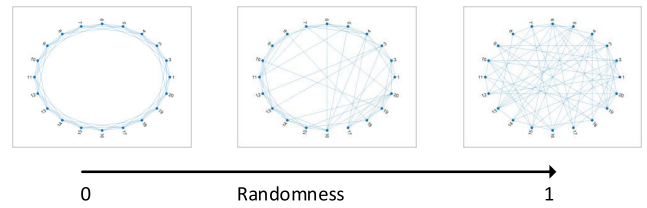
FIGURE 3. Rewiring of a network with probability 0 to 1 by applying the WS Small World Model. The regular network transforms to a random network by increasing the probability from 0 to 1.
