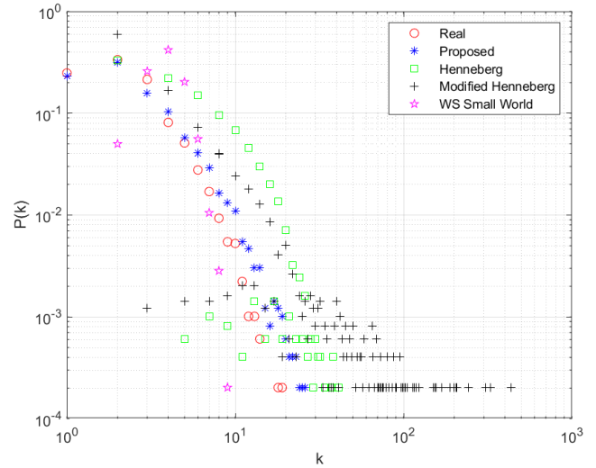
FIGURE 12. Degree Distribution of the real dataset (US Western States Power Grid), the proposed model, Henneberg's Model, Modified Henneberg's Model, and WS Small World Model.
