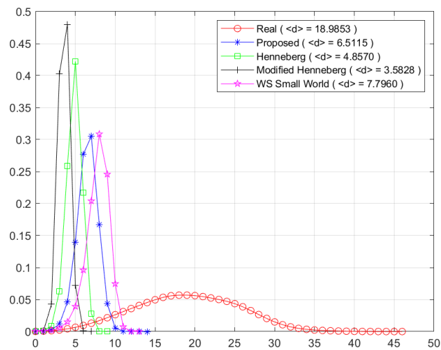
FIGURE 15. Distance Distribution of the real dataset (US Western States Power Grid), the proposed model, Henneberg’s Model, Modified Henneberg’s Model, and WS Small World Model. The legend in the graph shows the average path length of each network.
