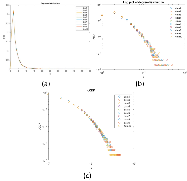
FIGURE 6. Simulation results of the 10 different runs of the proposed model. (a) Degree distribution of the proposed model. (b) Log plot of the Degree Distribution (c) cCDF of the proposed model for 10 different simulation runs.
