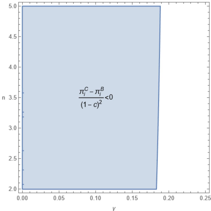
FIGURE 1 \pi_i^C - \pi_i^B for \tau = 2 , \rho = 0.8 , n \in [2, 5] and \gamma \in [0, 0.25] [Colour figure can be viewed at wileyonlinelibrary.com ]
