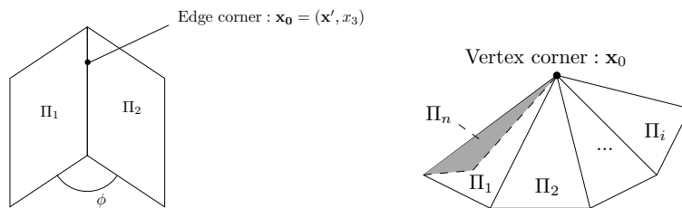
FIG. 1. Schematic illustrations of edge corner and vertex corner, respectively.
