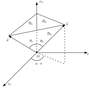
FIG. 3. Schematic illustration of a vertex corner that is intersected by \Pi_1 , \Pi_2 , and \Pi_3 .
