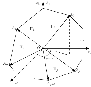
FIG. 4. Schematic illustration of a vertex corner that is intersected by \Pi_1, \Pi_2, \dots, \Pi_n with n > 3 .
