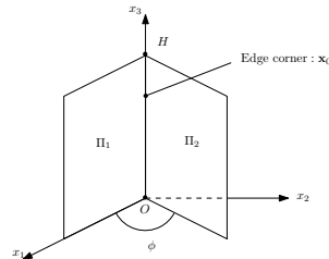
FIG. 2. Schematic illustration of two intersecting planes with an edge corner and the dihedral angle \phi .
