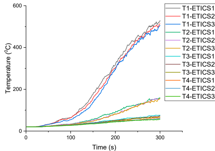
Figure 5. Variation in recorded temperature with time for the 3 scenarios of ETICS façade at Device T1, Device T2, Device T3 and Device T4.
