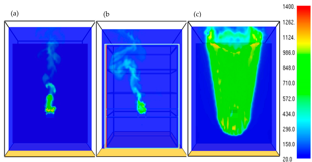
Figure 8. Vertical temperature distribution slice at simulation time 200 s of the scenarios (a) ETICS1, (b) DSF1, (c) VGS1.
