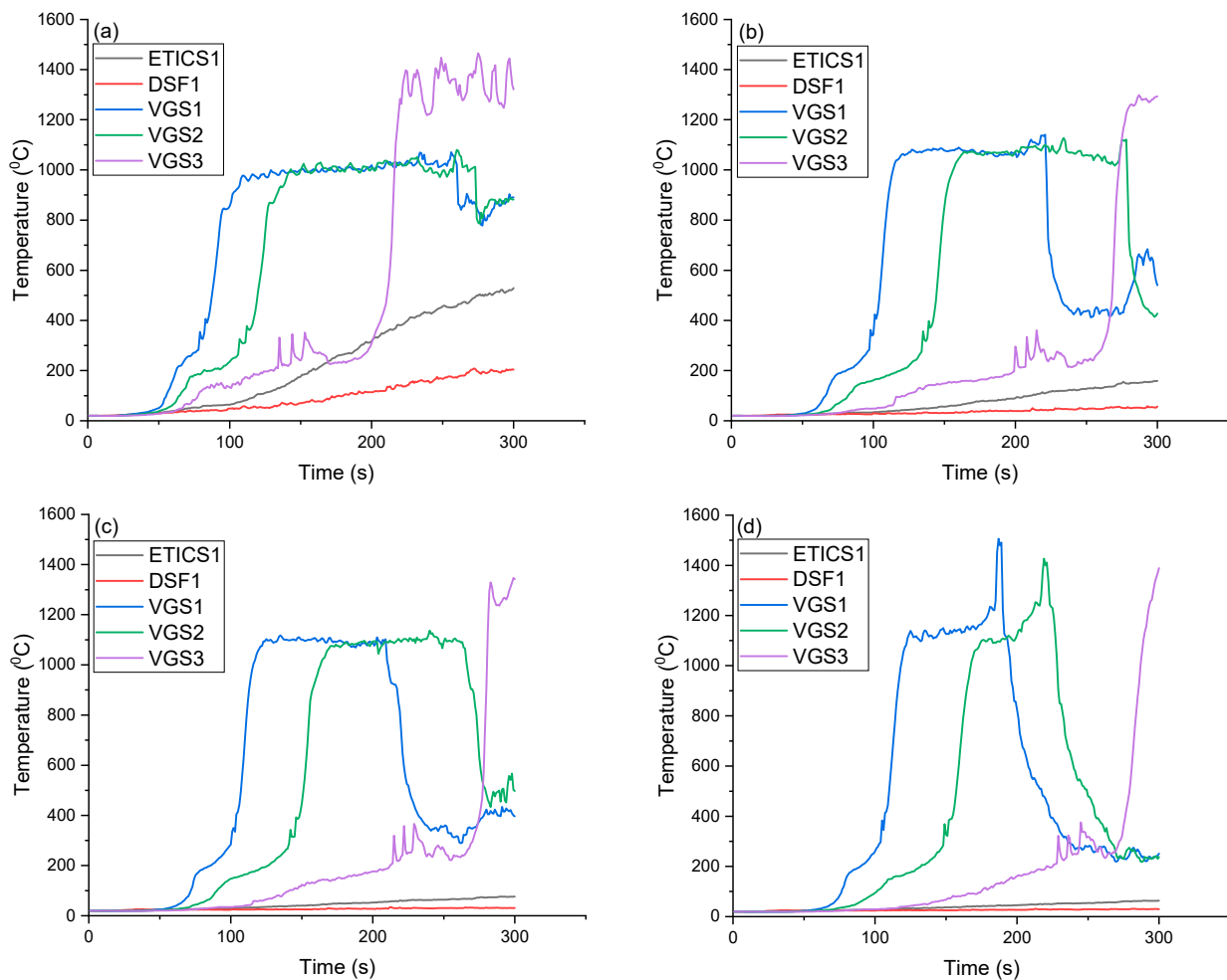
Figure 7. Variation in recorded temperature with time for the 3 scenarios of VGS along with ETICS1 and DSF1 at (a) Device T1, (b) Device T2, (c) Device T3 and (d) Device T4.
