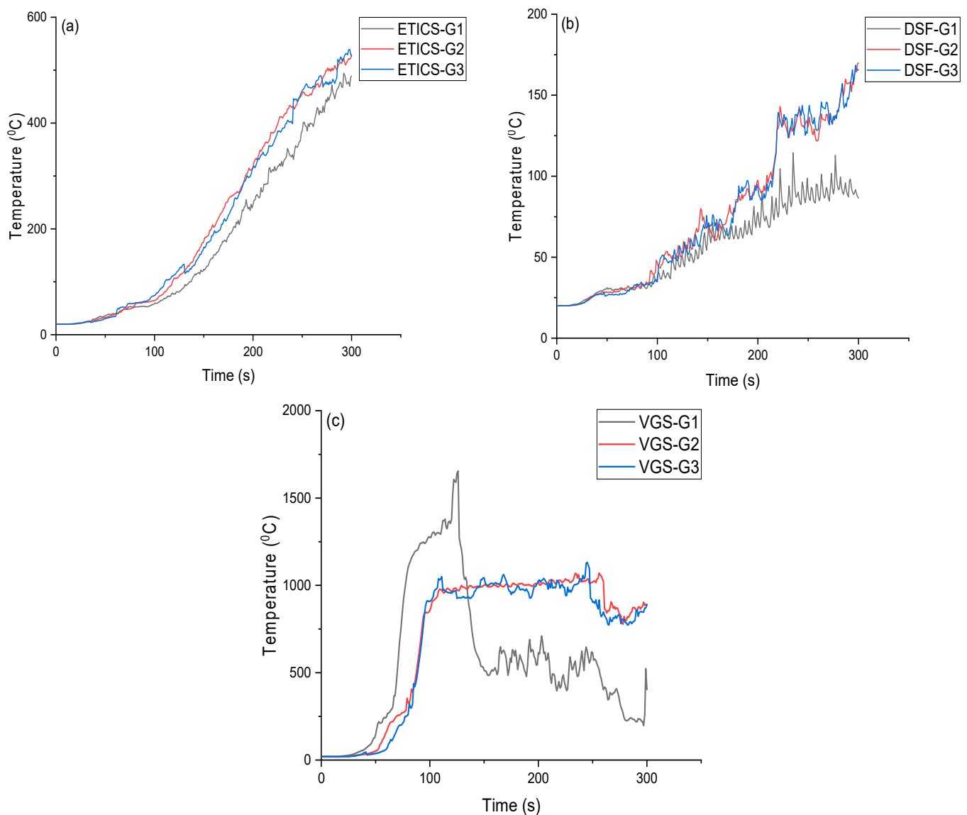
Figure 3. Grid sensitivity analysis of (a) ETICS, (b) DSF, (c) VGS.
