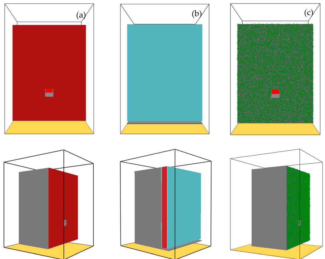
Figure 4. FDS building model of (a) ETICS façade, (b) DSF, (c) VGS wall.
