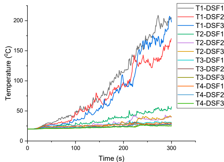
Figure 6. Variation in recorded temperature with time for the 3 scenarios of DSF at Device T1, Device T2, Device T3 and Device T4.
