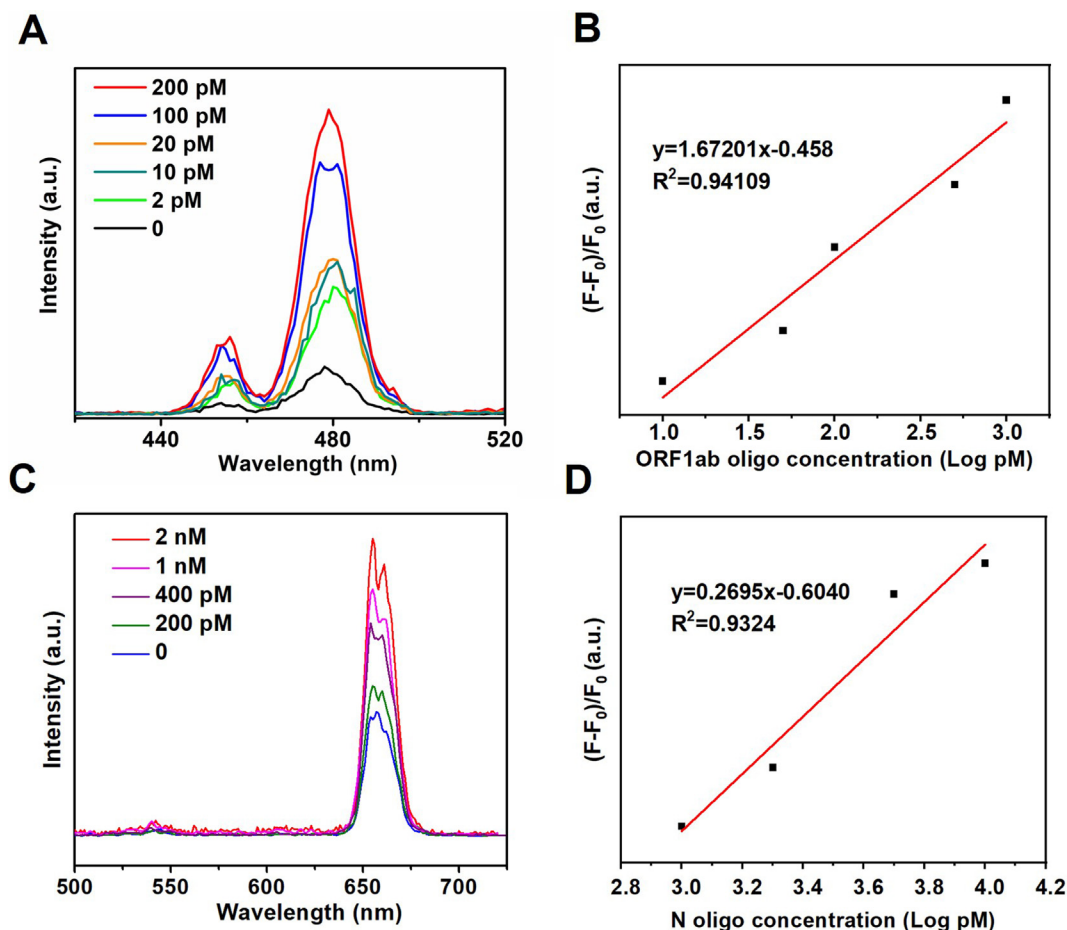
Fig. 3. (A and B) UC emission spectra of the Nb 2 CT x /blue-emitting UCNP assay in the presence of different concentrations of short ORF1ab target. (C and D) UC emission spectra of the Nb 2 CT x /red-emitting UCNP assay in the presence of different concentrations of short N -gene target. (For interpretation of the references to color in this figure legend, the reader is referred to the web version of this article.)
