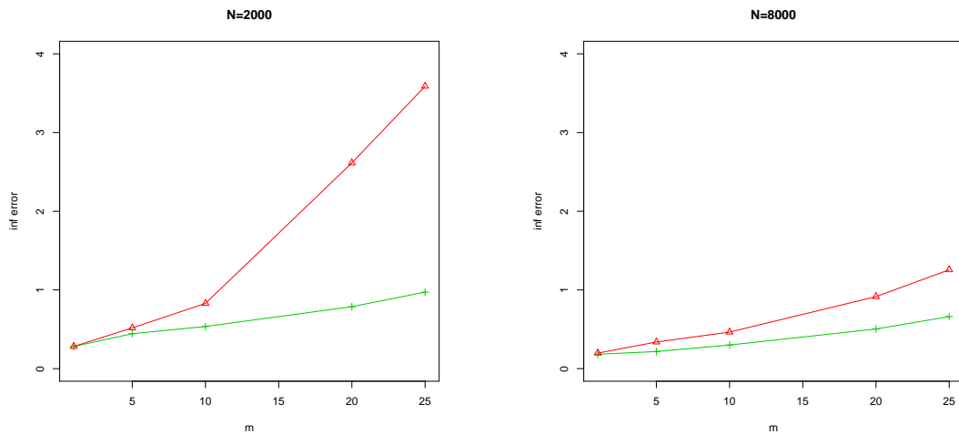
Figure 2: The l_\infty errors of estimates with m \in \{1, 5, 10, 20, 25\} ( m = 1 represents the centralized estimator). \triangle (red): naive aggregated estimator (NAI); + (green): the aggregated estimator after debiasing (ABC). Left panel: n = 2000 , right panel: n = 8000 .
