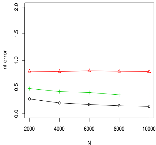
Figure 3: The l_\infty errors of estimates with p = 1000 and N \in \{2000, 4000, 6000, 8000, 10000\} . \circ (black): centralized estimator (CEN); \triangle (red): naive aggregated estimator (NAI); + (green): the aggregated estimator after debiasing (ABC).
