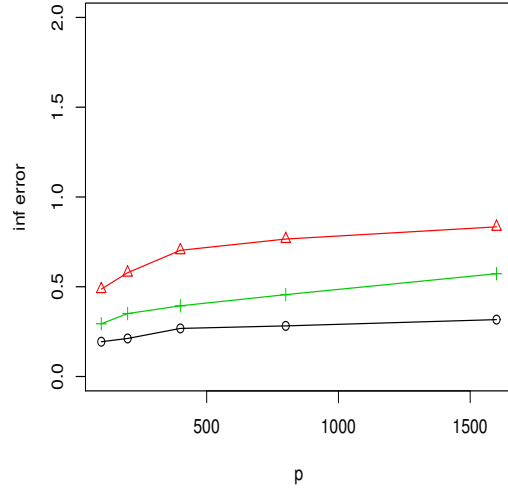
Figure 1: The l_\infty errors of estimates with changing dimension p . \circ (black): centralized estimator (CEN); \triangle (red): naive aggregated estimator (NAI); + (green): the aggregated estimator after debiasing (ABC).
