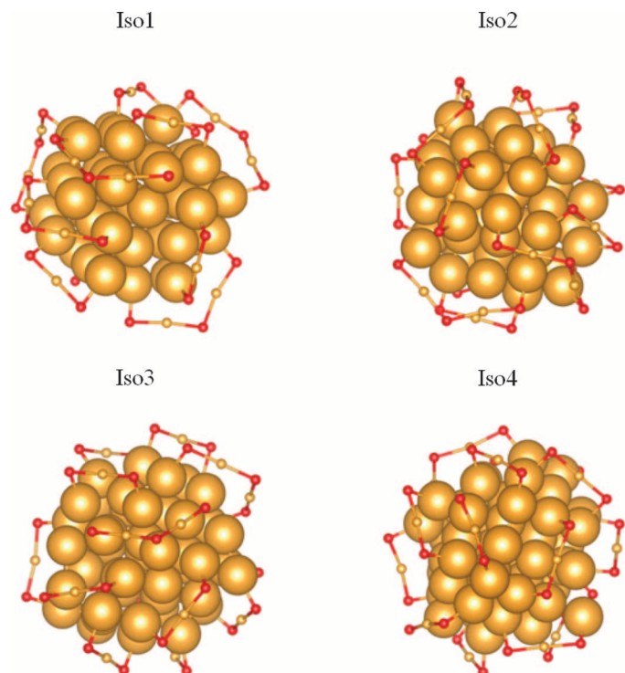
Fig. 1. Optimized structures of the four isomers Iso1 to Iso4 of \text{Au}_{68}(\text{SH})_{32} . The Au and S atoms are in gold and red, respectively. The H atoms are not shown.
